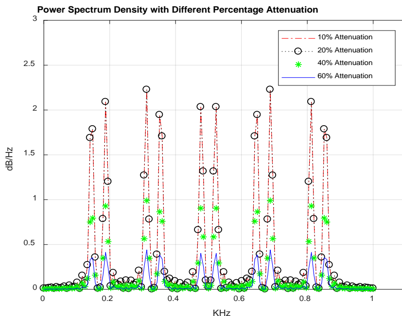
Fig.8: Power Spectrum Density with Different Percentages of Attenuations
