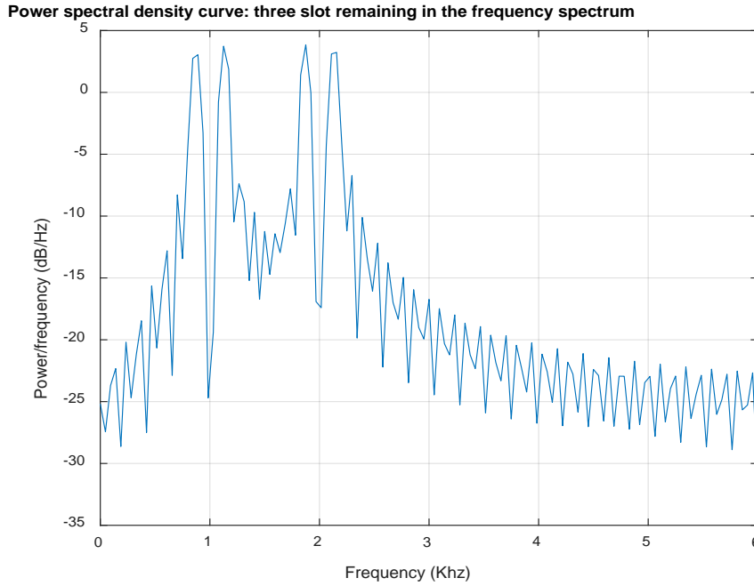
Fig.5: Power Spectrum Density Curve: Three Slots remaining in the frequency Spectrum Effective Use of Spread Spectrum with SUs QoS Enabled
