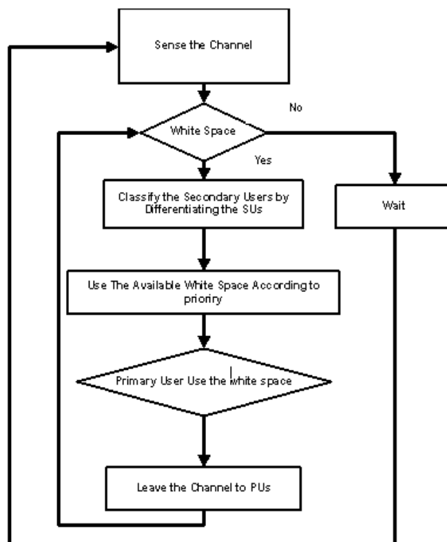
Fig.3: Proposed Cognitive Radio with Differentiated QoS
