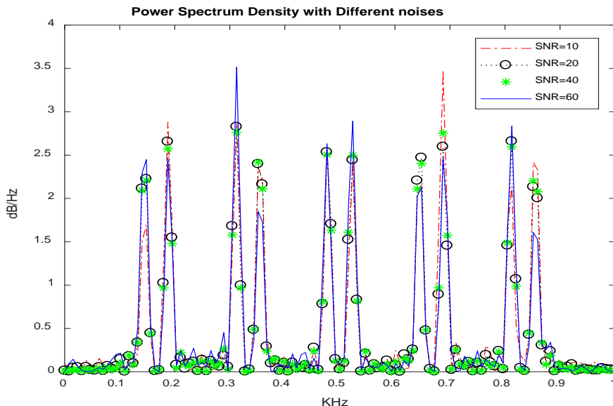
Fig.7: Power Spectrum Density with Different Added Noises
