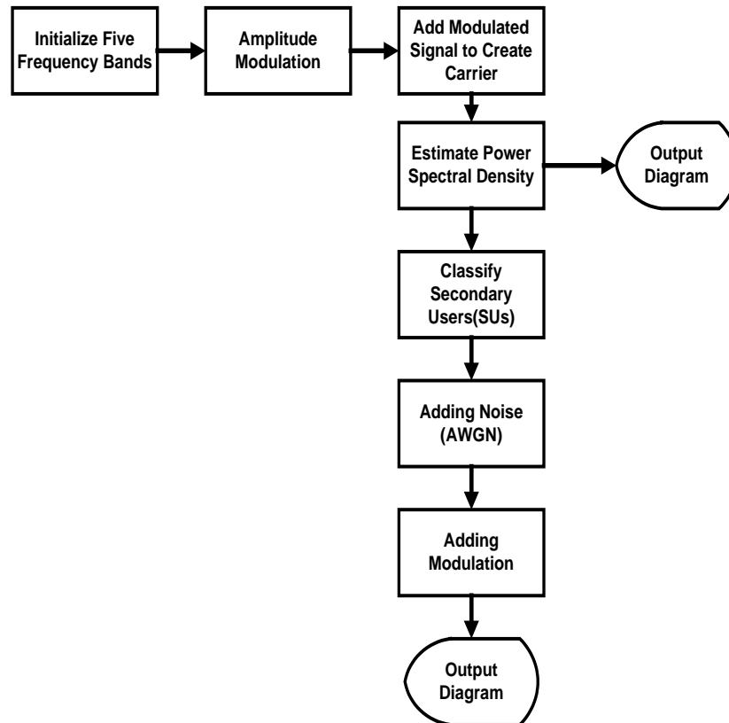
Fig.4: Block Diagram for Cognitive Radio with Differentiated QoS
