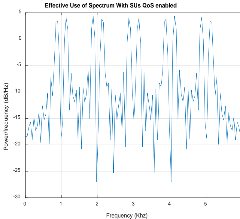
Fig.6: Fully Utilized Spectrum with SUs QoS Enabled Noise Effect on Spread Spectrum Density
