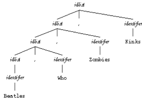
Fig. 2: Nested Identifiers
