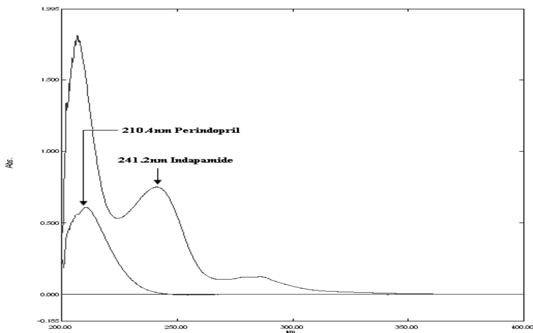
Fig 3. Overlain spectra of perindopril ( 40 \mu\text{g mL}^{-1} ) with a maximum at 210.4 nm and indapamide ( 12.5 \mu\text{g mL}^{-1} ) with a maximum at 241.2 nm in methanol taken on UV – Vis spectrophotometer (SHIMADZU 1700)
