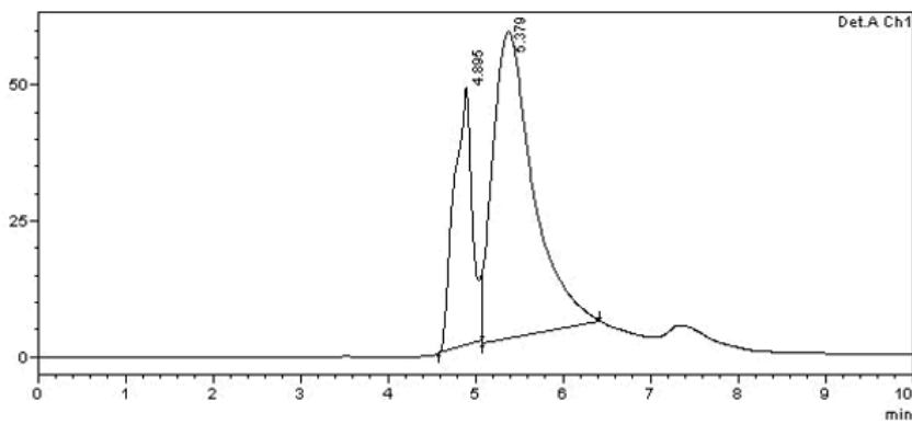
Fig.3: Chromatogram of Blank Plasma
