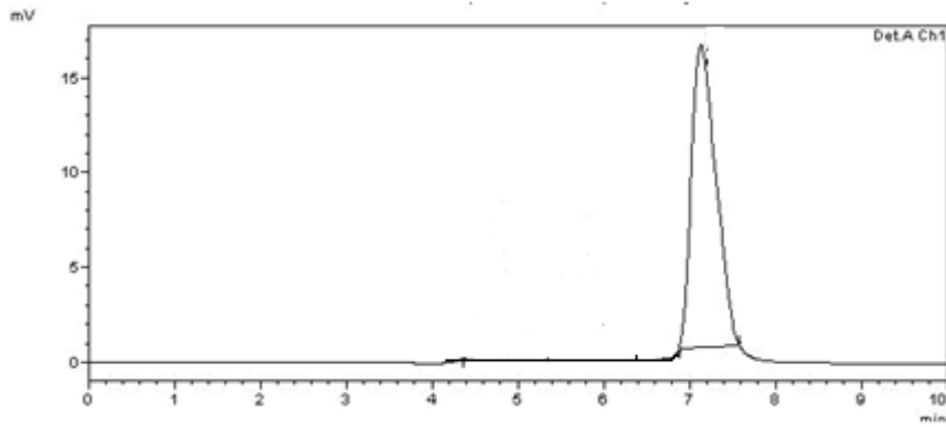
Fig.2: Chromatogram of Valacyclovir HCL in Plasma
