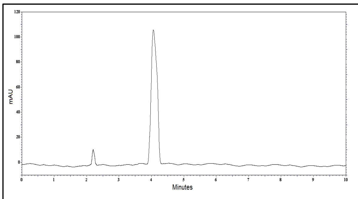
Figure 6. HPLC chromatogram of photolytic degradation behavior of tetramisole hydrochloride after exposing to sunlight for 48 hours
