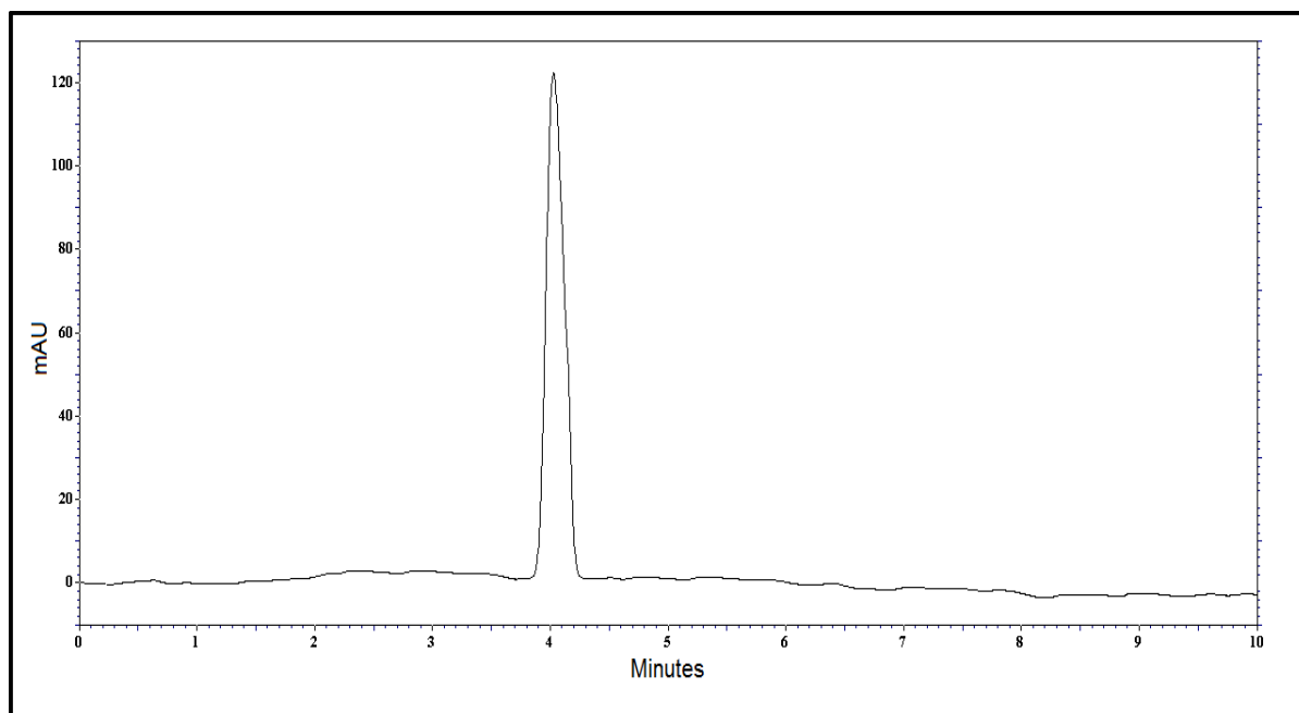
Figure 2. HPLC chromatogram of 5 µg/mL tetramisole hydrochloride at 212 nm
