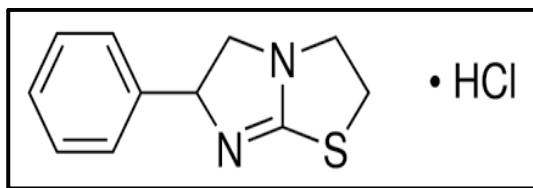
Figure 1. Chemical structure of tetramisole hydrochloride
