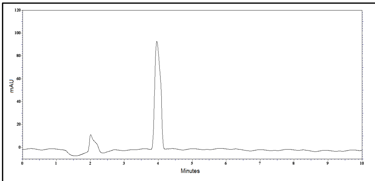
Figure 3. HPLC chromatogram for acidic hydrolysis of tetramisole hydrochloride after exposure to 0.1 N HCl for 24 hr. at ambient temperature
