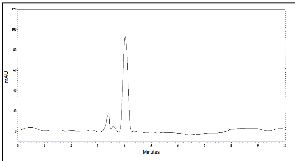
Figure 5. HPLC chromatogram of oxidative degradation behavior of tetramisole hydrochloride after exposing to 3 % H 2 O 2 for 6 hour at ambient temperature
