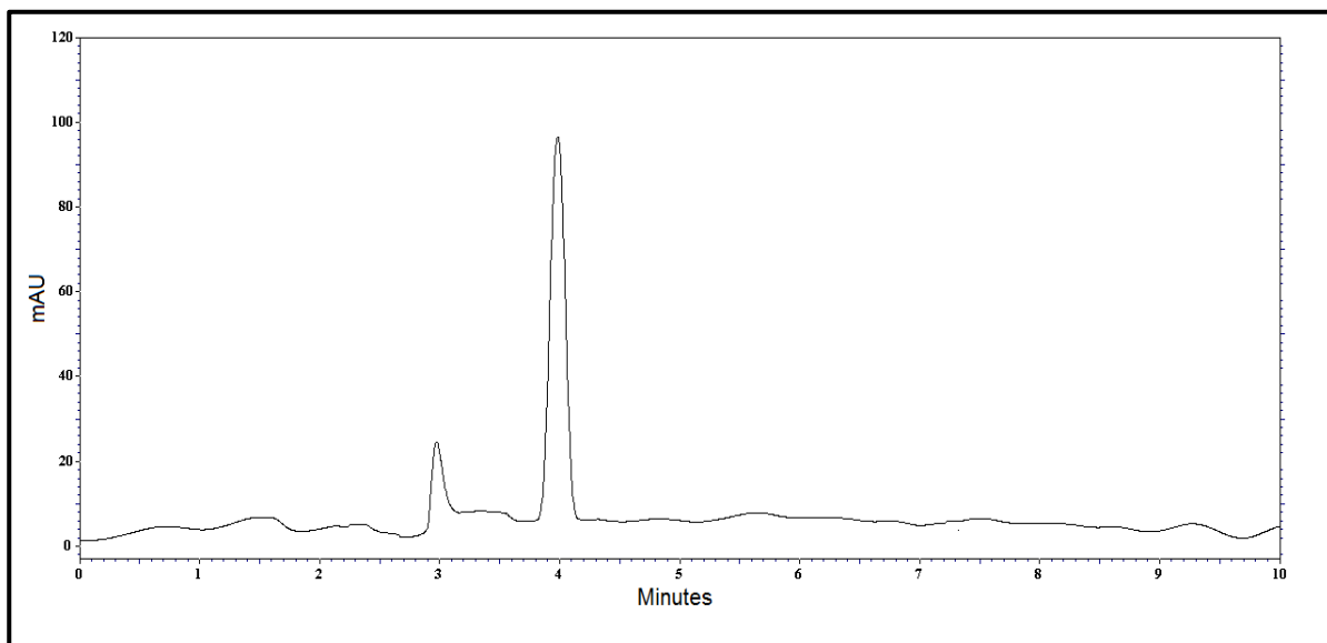
Figure 4. HPLC chromatogram for basic hydrolysis of tetramisole hydrochloride after exposure to 0.1 N NaOH for 4 hr. at ambient temperature
