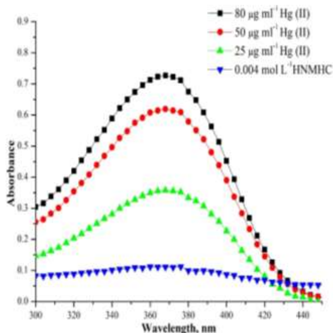
Figure 1: Absorption spectra of Hg(II)- HNMHC complex
