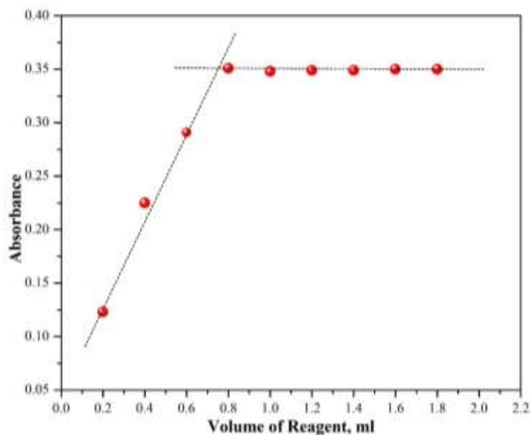
Figure 8: Mole ratio method for Hg (II)- HNMHC complex
