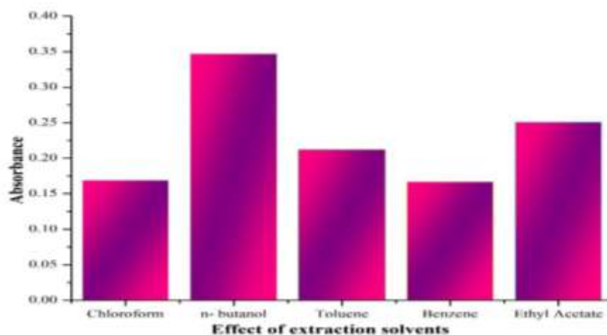
Figure 4: Effect of extraction solvents on Hg (II)- HNMHC
