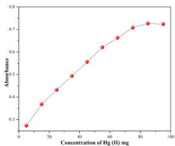
Figure-6: Ringbom's Plot of Bi (III)- HNMHC complex
