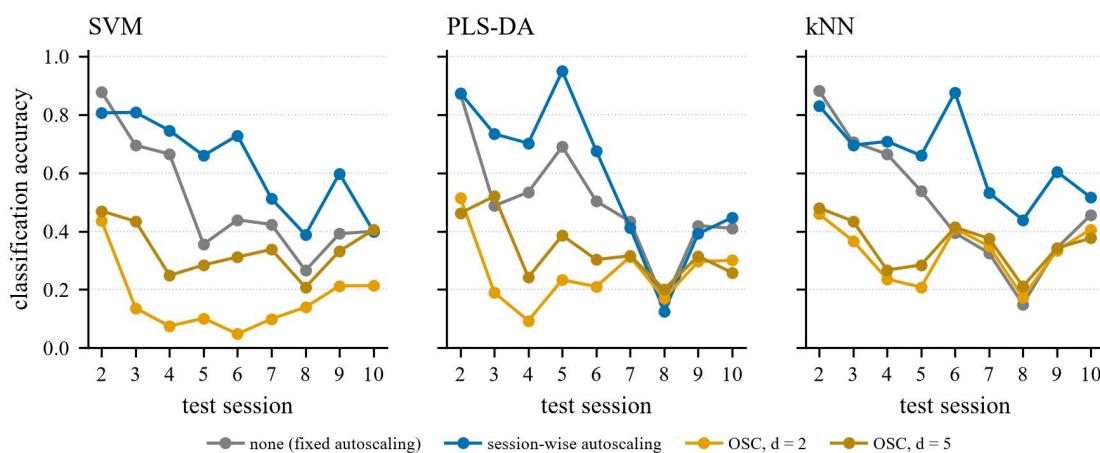
Fig. 6 Protocol I. Accuracy on each test session for a model calibrated on session 1 only, using the signed-log transform, for the three classifiers and four correction strategies
