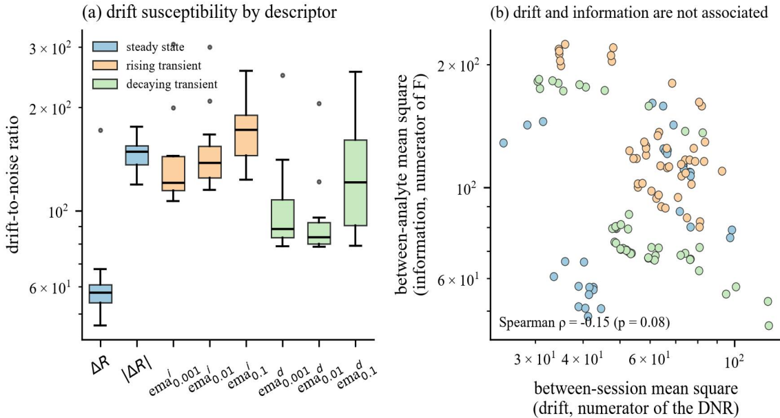
Fig. 5 Drift susceptibility of the descriptors. (a) Distribution over the sixteen sensor units of the drift-to-noise ratio of each descriptor type, on a logarithmic scale, shaded by descriptor family. (b) The two numerators compared directly, the between-analyte mean square of equation (8) against the between-session mean square of equation (4), so that the within-cell mean square they share cannot induce an association; drift susceptibility and analyte-discriminating power are not positively related
