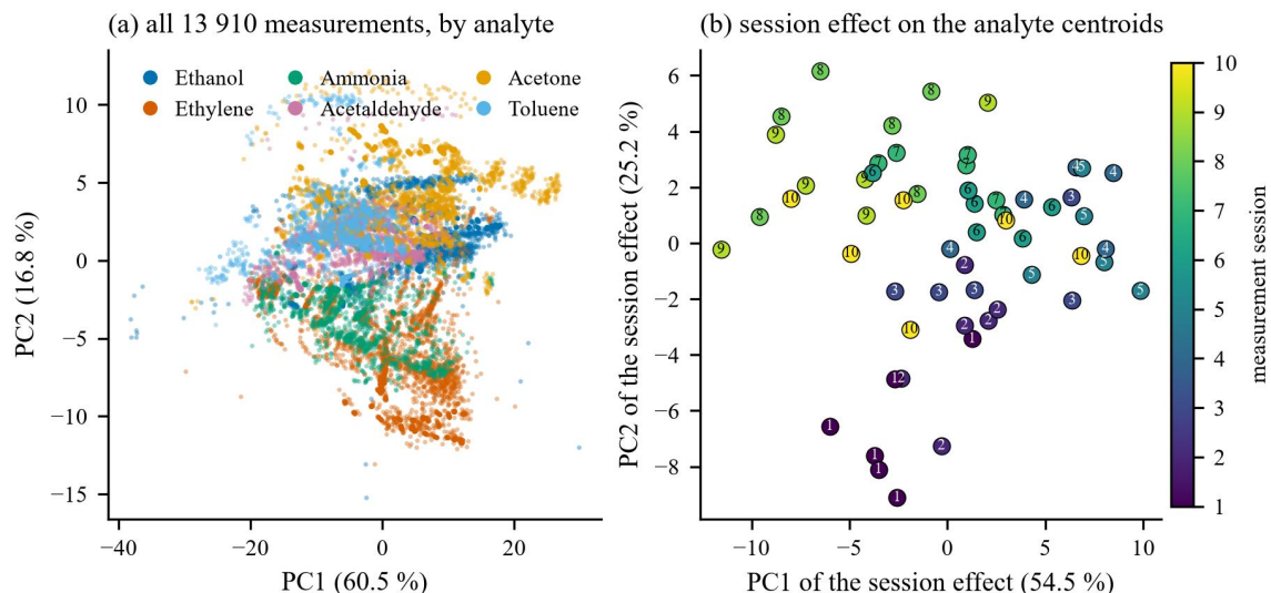
Fig. 3 Principal component analysis of the signed-log transformed, autoscaled archive. (a) All 13 910 measurements, coloured by analyte. (b) Session effect: centroid of each analyte in each session after removal of the analyte main effect, coloured and labelled by session index. Measurements made in the same session move together regardless of which analyte was dosed
