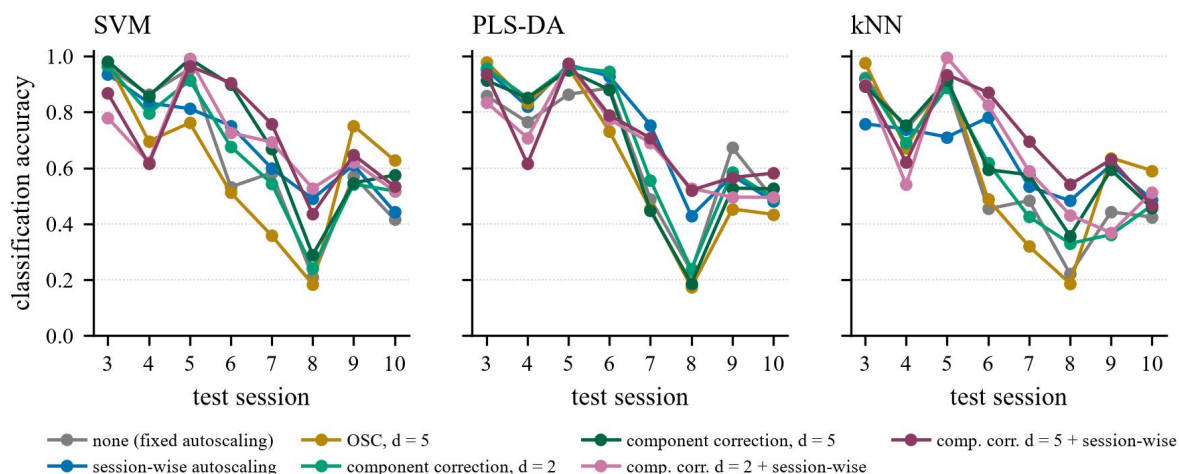
Fig. 7 Protocol II. Accuracy on each test session for a model calibrated on sessions 1 and 2, using the signed-log transform, for the three classifiers and seven correction strategies
