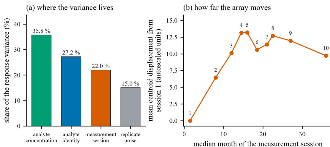
Fig. 2 Structure and magnitude of the drift. (a) Share of the response variance carried by the analyte concentration, the analyte identity, the measurement session and the replicate noise, from the decomposition of equation (7). (b) Mean displacement of the analyte centroids with respect to session 1, in autoscaled units, against the median month of each session; the labels give the session index
