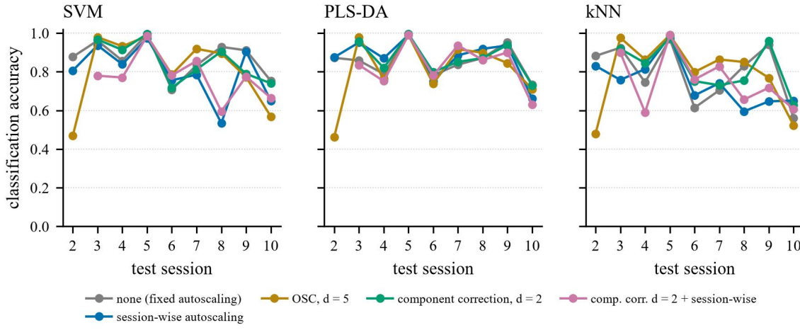
Fig. 9 Protocol III. Accuracy on session k for a model calibrated on all sessions up to k-1 , using the signed-log transform, for the three classifiers and the main correction strategies
