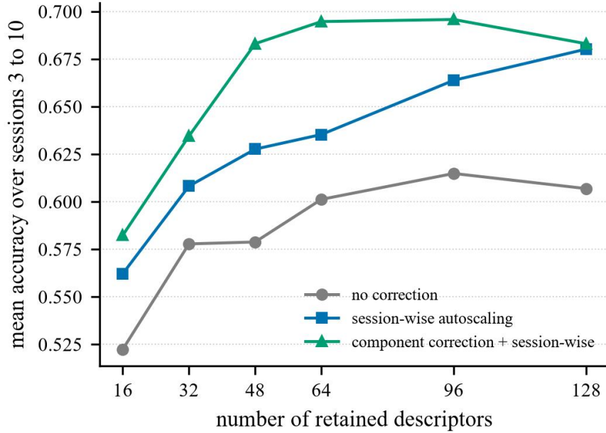
Fig. 8 Protocol II. Mean accuracy over test sessions 3 to 10 against the number of descriptors retained by the drift-to-noise criterion, averaged over the six combinations of signal transform and classifier, for three correction strategies
