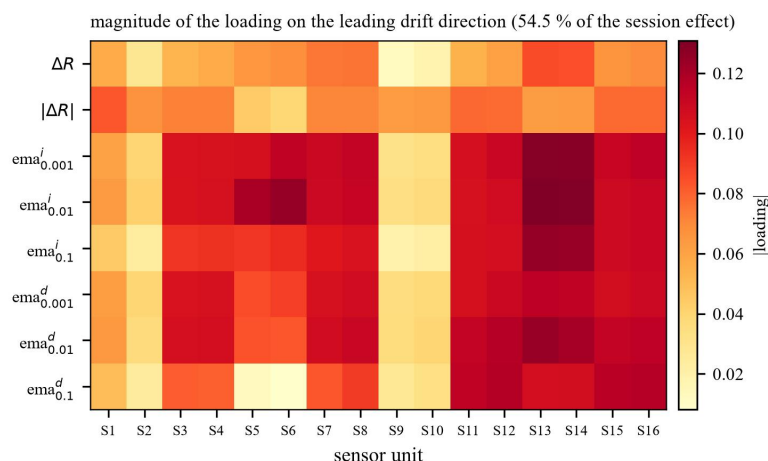
Fig. 4 Magnitude of the loading of each of the 128 descriptors on the leading direction of the session effect, arranged by sensor unit and descriptor type. Darker cells carry more of the drift
