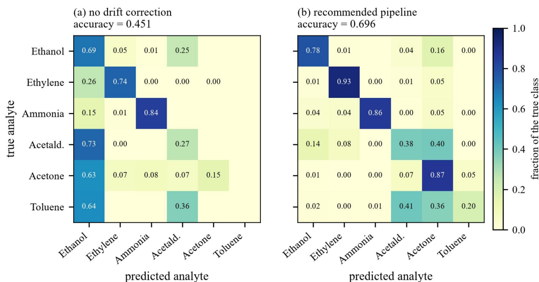
Fig. 10 Confusion matrices pooled over test sessions 3 to 10 under Protocol II, normalised by the number of measurements of each true analyte, for (a) the uncorrected reference pipeline and (b) the recommended corrected pipeline
